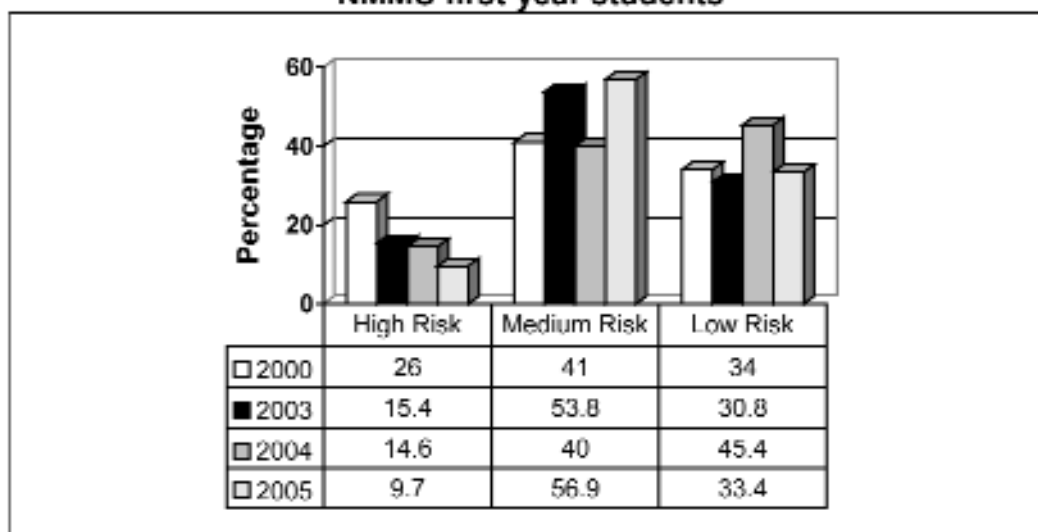
Figure 3: Percentages per risk profile for the 2000, 2003 and 2005 intakes of NMMU first-year students
