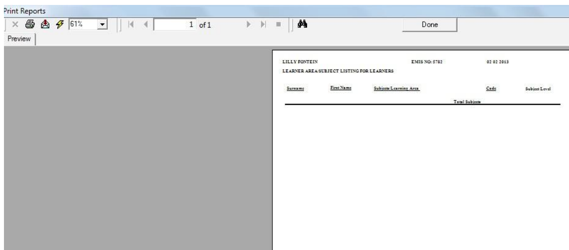
Figure 48: Print Reports
