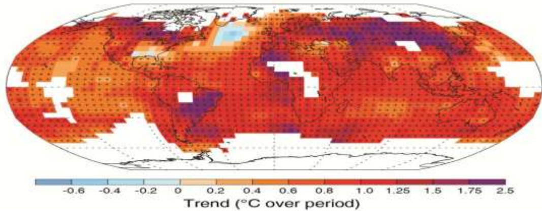
(b) Observed change in average surface temperature 1901–2012
