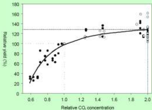
Wheat yields with increasing CO 2 concentration
