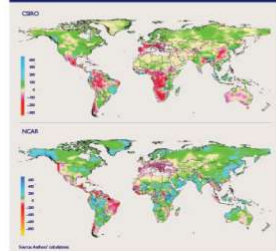
Figure 2—Change in precipitation (mm), 2000–2050
