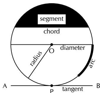
Figure 9.1: Parts of a circle
