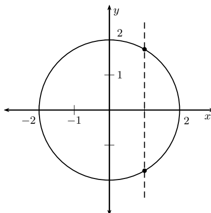
Figure 6.1: Graph of x^2 + y^2 = 4
