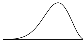
Skewed left
