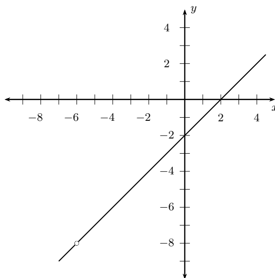
Figure 7.1: Graph of y = \frac{(x+6)(x-2)}{x+6} .
