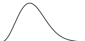
Skewed right
