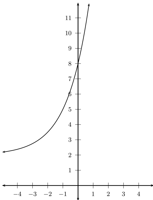
Figure 13.2: Graph of g(x) = 3 \cdot 2^{x+1} + 2 .
