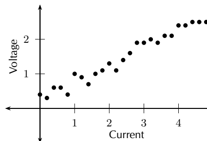
Figure 18.4: Example of a scatter plot
