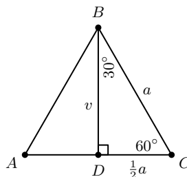
Figure 17.8: An equilateral triangle with one angle bisected.
