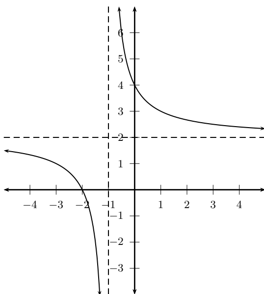
Figure 12.2: Graph of g(x) = \frac{2}{x+1} + 2 .
