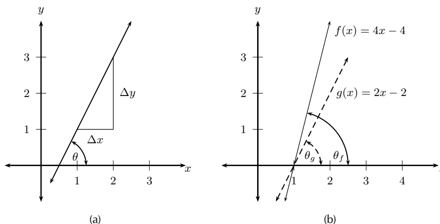
Figure 16.4: (a) A line makes an angle \theta with the x -axis. (b) The angle is dependent on the gradient. If the gradient of f is m_f and the gradient of g is m_g then m_f > m_g and \theta_f > \theta_g .
